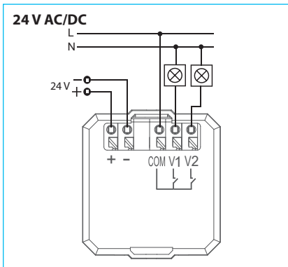
The output contacts (V1, V2) are galvanically isolated from the power supply and share a common COM terminal
