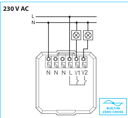
The output contacts (V1, V2) switch the phase potential (L) and are equipped with zero cross switching technology
