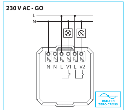
Output contact V1 is at the same potential as the product power supply. Output contact V2 is separate from the power supply but must be connected to the same potential. The wiring is used when it is necessary to secure V1 and V2 separately.
